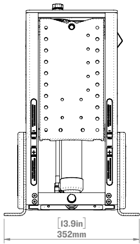
WITH SW-03620 DECK MOUNT
