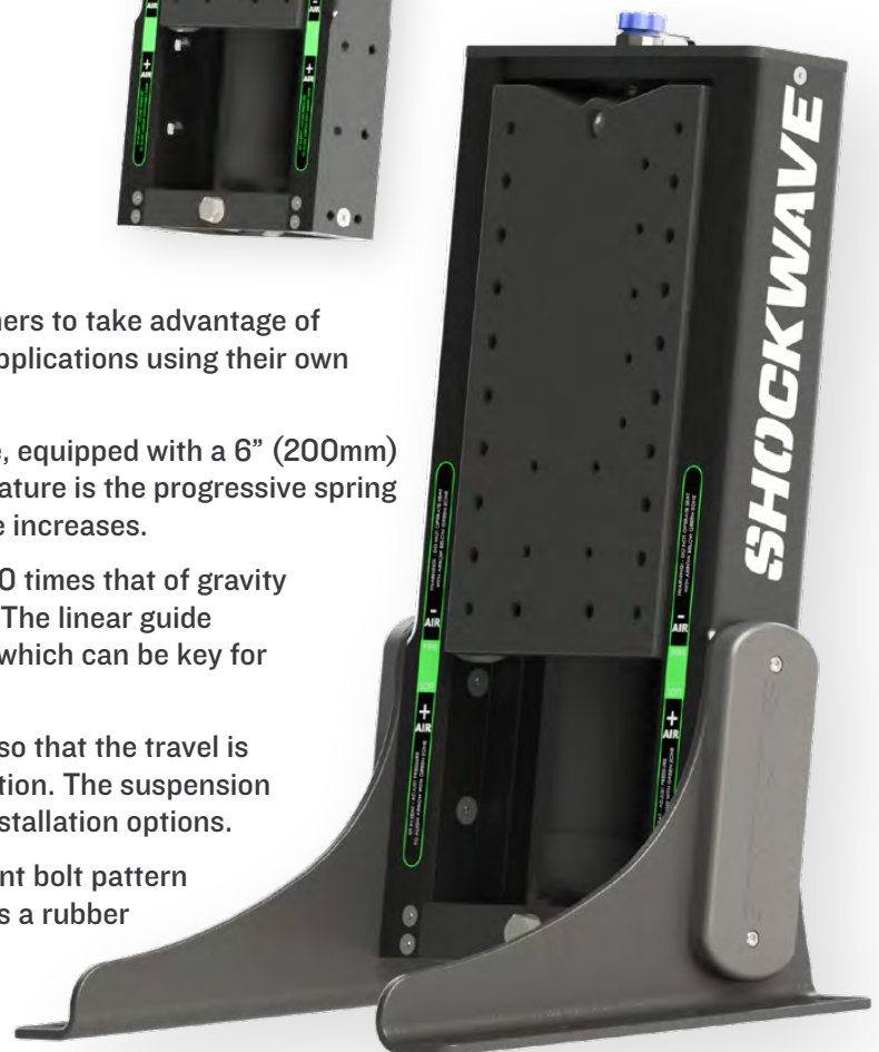
S2 module shown with deck mount
