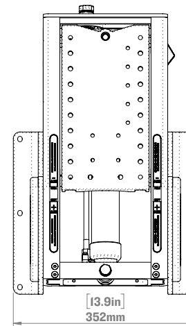
WITH SW-04871 10 DEGREE BULKHEAD MOUNT
