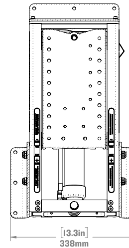
WITH SW-04656 0 DEGREE BULKHEAD MOUNT
