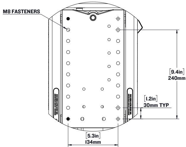
DETAIL A SCALE 1 : 6
