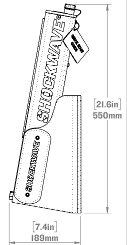
WITH SW-04871 10 DEGREE BULKHEAD MOUNT
