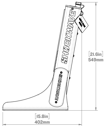
WITH SW-03620 DECK MOUNT
