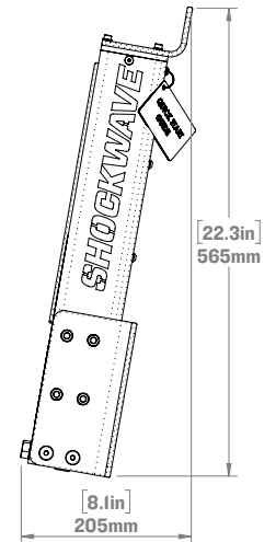
WITH SW-04656 0 DEGREE BULKHEAD MOUNT
