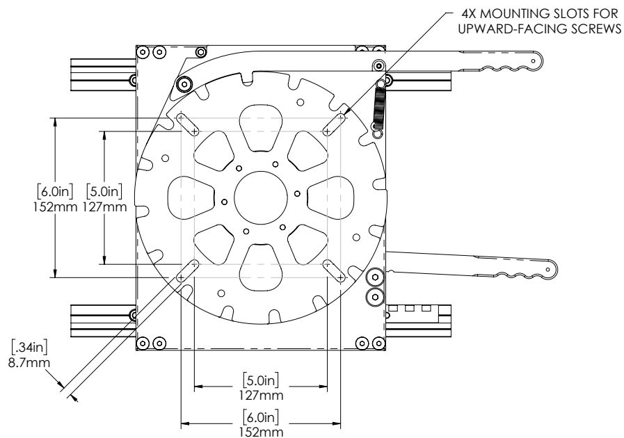
MOUNTING PATTERN FOR UPWARD-FACING SCREWS
