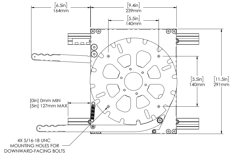
MOUNTING PATTERN FOR DOWNWARD-FACING SCREWS
